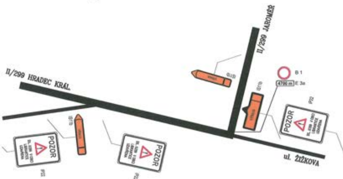
DETAIL 6.
